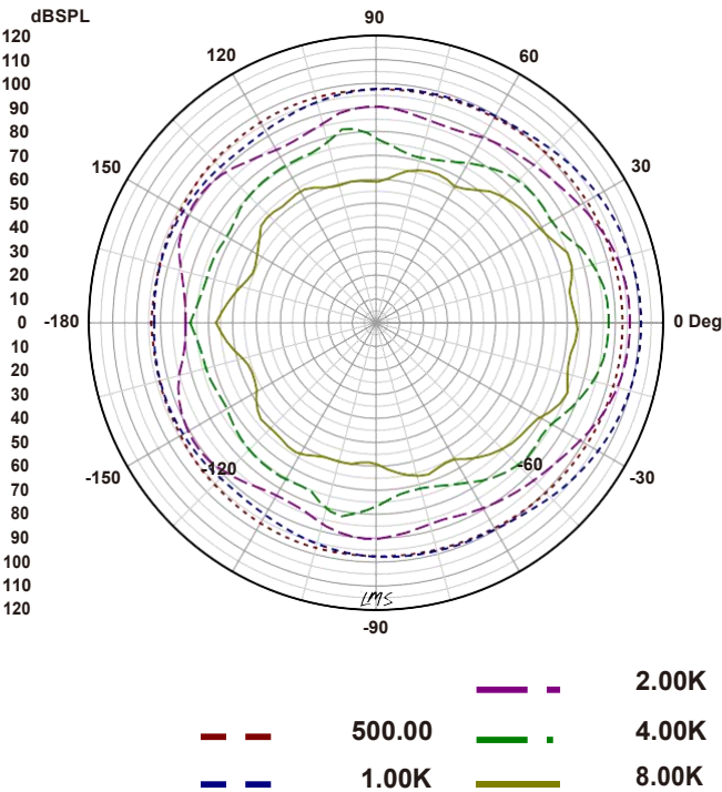
Directive pattern
