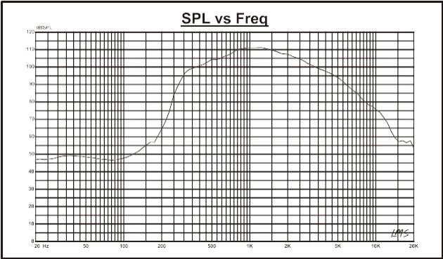
Frequency response diagram
