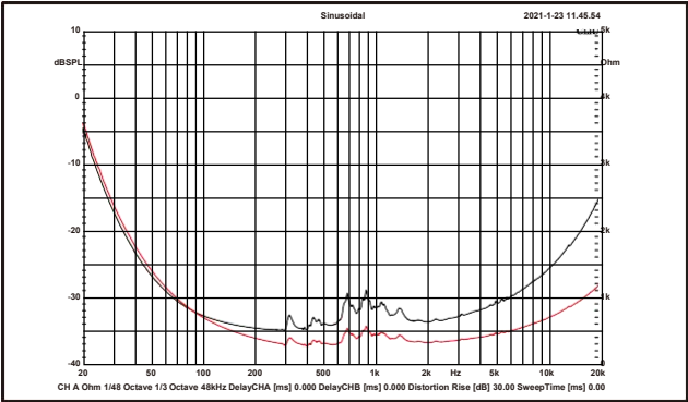
Impedance diagram
