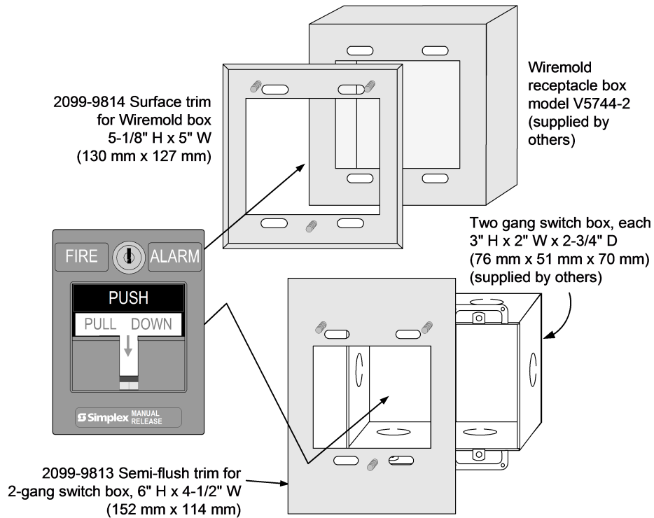
Figure 6: Additional mounting information
