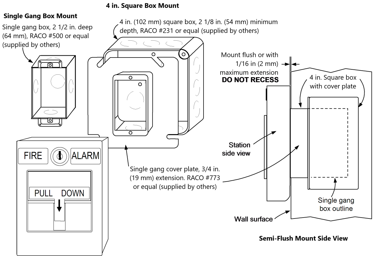
Figure 3: Semi-flush mounting reference
